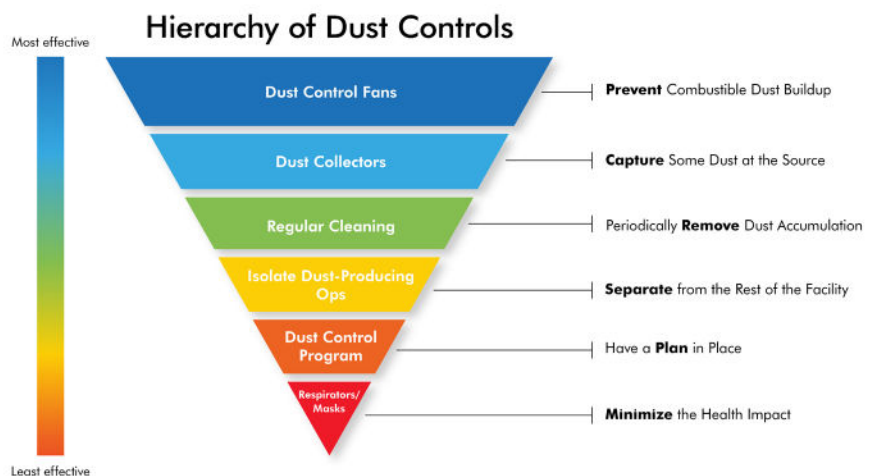
FIGURE 1: Hierarchy of Dust Control Technologies
