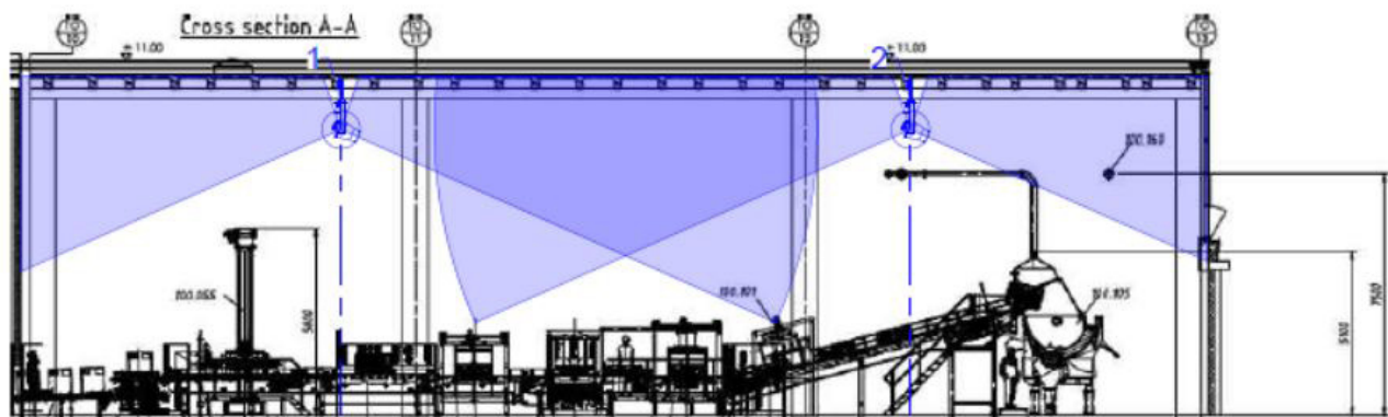
FIGURE 3: Typical horizontal application of a DPC robotic fan system.
