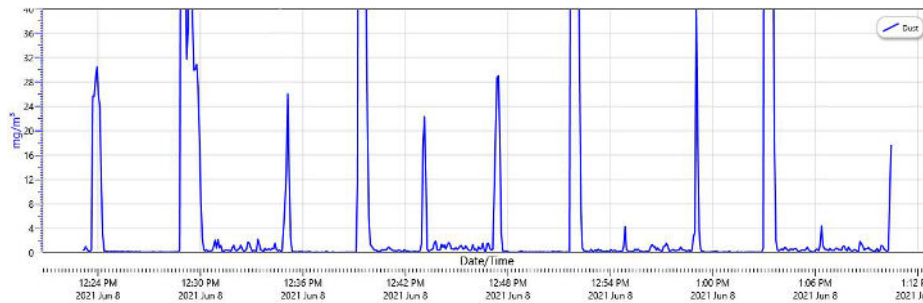
FIGURE 5: Measured total particulate levels WITHOUT robotic fan system in operation.
