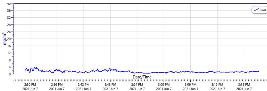
FIGURE 6: Measured total particulate levels WITH SonicAire fans in operation.
