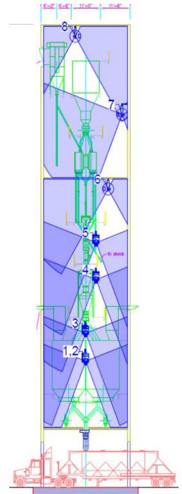
FIGURE 4: Typical layout of a vertical DPC robotic fan system in an agricultural application.
